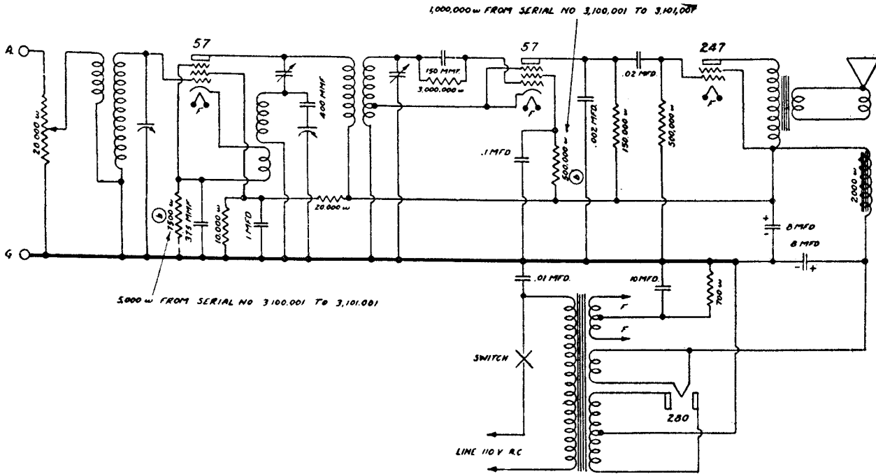
SCHEMATIC DIAGRAM
